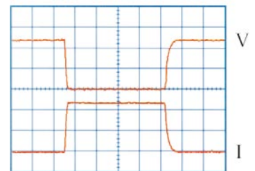
Very fast pulse rise and fall times ( <1\mu\text{s} ), and low ripple, produce a nearly ideal, flat-top pulse like this 20kV, 100A, 1\mu\text{s/cm} . Upper trace voltage, lower trace current.
